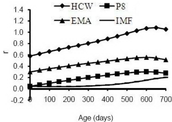
Figure 4. Phenotypic correlations between live weight and carcass traits over time. HCW = hot carcass weight; P8 = rump fat depth.
