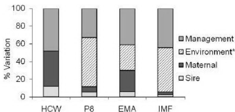
Figure 3. Relative contribution to variation in carcass quality traits. *For carcass traits, environment includes permanent + temporary environmental. For abbreviations, see legend to Table 2.
