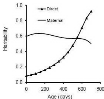
Figure 2. Estimates of additive and dam heritabilities over time.
